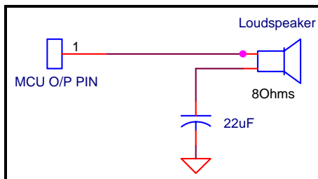
Figure 5. Direct Loudspeaker Drive Arrangement
